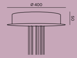
Canopy also for PWM dimming system
